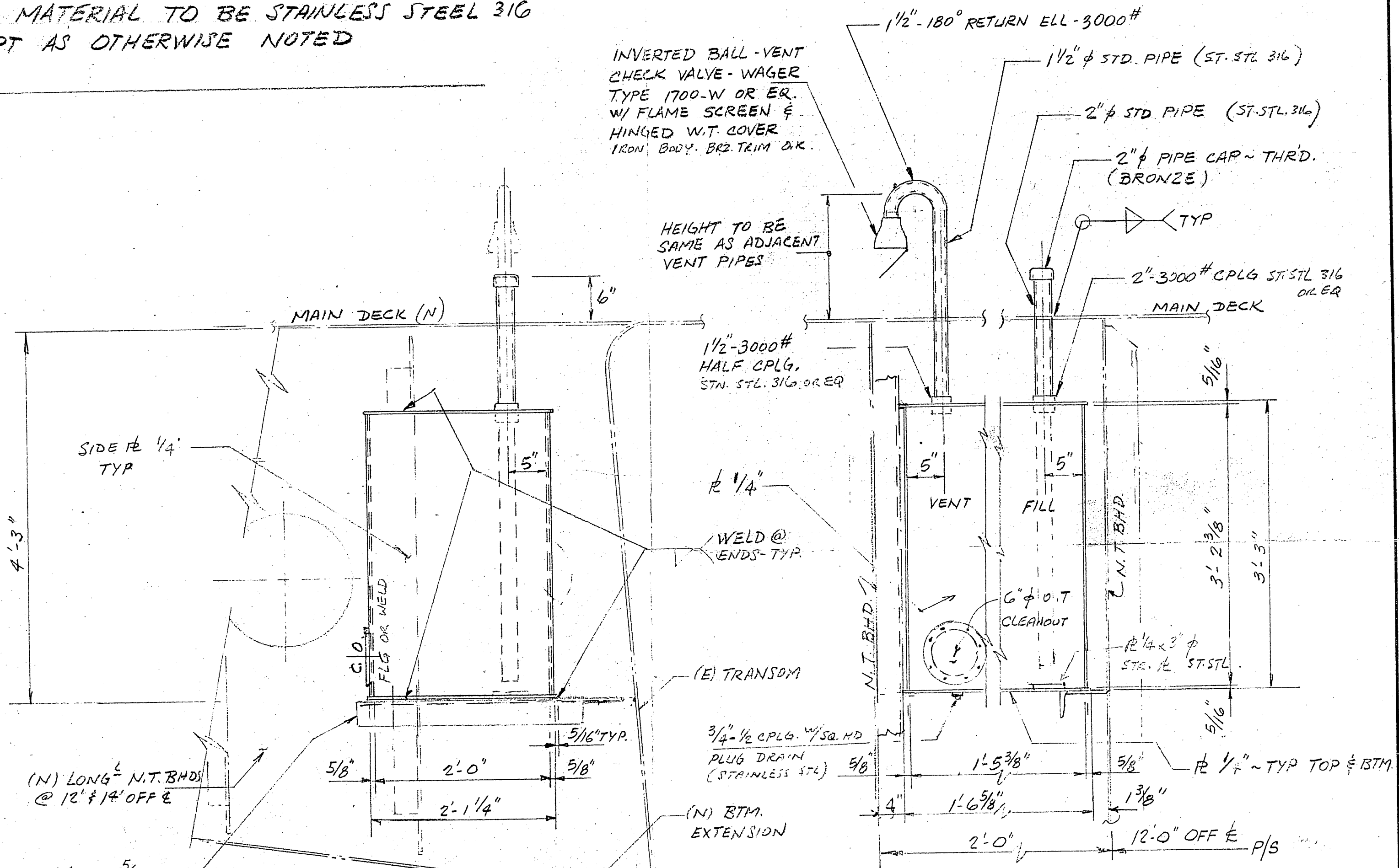
SECTION "1-A" LKG. FWD. 1" = 1'-0"
